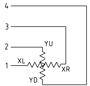
PIN ASSIGNMENT
