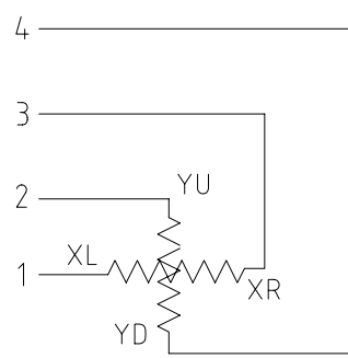
PIN ASSIGNMENT
